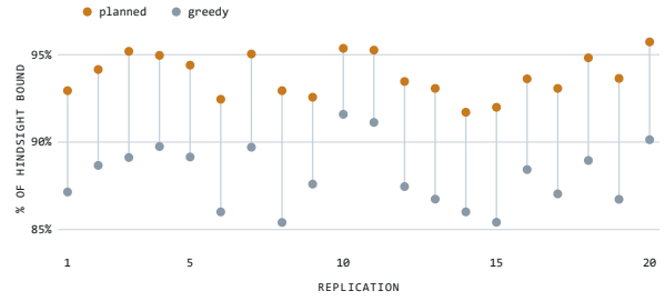
Figure 3. Revenue captured by each policy as a share of the hindsight offline optimum, per replication. Planned allocation dominates greedy serving in all 20 replications; the two distributions do not overlap (planned minimum 91.7%, greedy maximum 91.6%).
