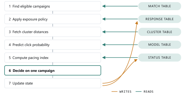
Figure 5. The seven-step decision path and its data dependencies. Steps 1–5 each read one pre-computed or live table; step 6 is pure arithmetic over the candidates; step 7 writes the served impression back into the status and response tables, which is also the record that feeds the next offline refinement cycle.
