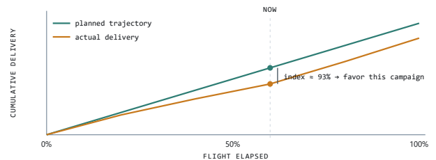
Figure 6. Pacing as trajectory tracking. The plan implies a cumulative delivery path; actual delivery drifts below it, the performance index measures the gap at the current moment, and the decision rule favors the lagging campaign on suitable impressions until the curves reconverge.
